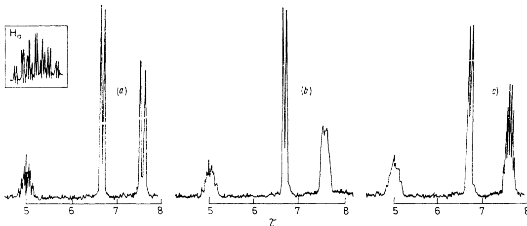
FIGURE 1 1 H N.m.r. spectra of (1-3- \eta -allyl)tris(trifluorophosphine)rhodium(I) at (a) room temperature, (b) -20, and (c) -50 °C in CCl_3F solution
