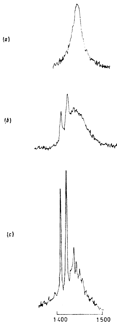
FIGURE 2 High-field half of ^{19}\text{F} n.m.r. spectra of the complex [\text{Rh}(\eta\text{-allyl})(\text{PF}_3)_3] at (a) room temperature, (b) -20^\circ , and (c) -50^\circ\text{C} in toluene solution. The scale is in Hz relative to \text{CCl}_3\text{F}
